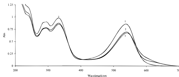
Figure 1. Electronic absorption spectra of 4 ( 4.05 \times 10^{-5} M, T = 25 °C) in aqueous solution. 1, pH 0.8; 2, pH 1.35; 3, pH 2.4.
