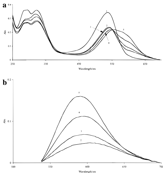
Figure 2. Electronic absorption spectra of 3 ( 1.8 \times 10^{-5} M, T = 25 °C) in aqueous solution, before (a) and after (b) the subtraction of the flavylium cation absorption. 1, pH 0.8; 2, pH 1.6; 3, pH 2.0; 4, pH 2.8; 5, pH 3.5.
